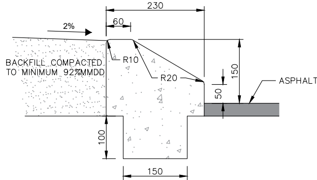
10 Semi-Mountable Kerb (Keyed) Type SMK2
