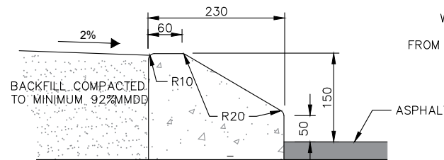
9 Semi-Mountable Kerb Type SMK1
