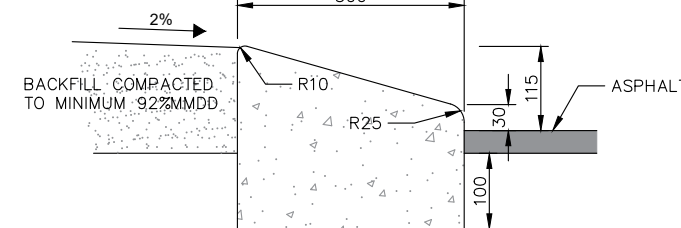
7 Mountable Kerb (Keyed) Type MK3
