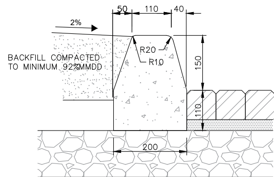
3 Barrier Kerb with Brickpaving Type BK3
