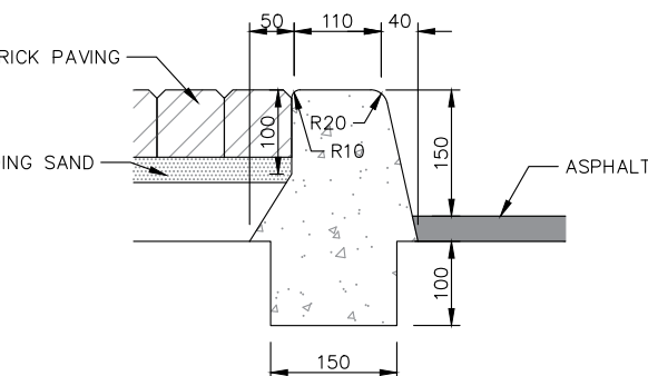
4 Barrier Kerb with Brickpaving (Keyed) Type BK4
