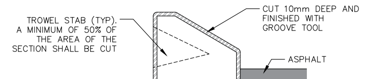
14 Contraction Joint Detail
