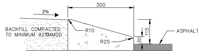
5 Mountable Kerb Type MK1
