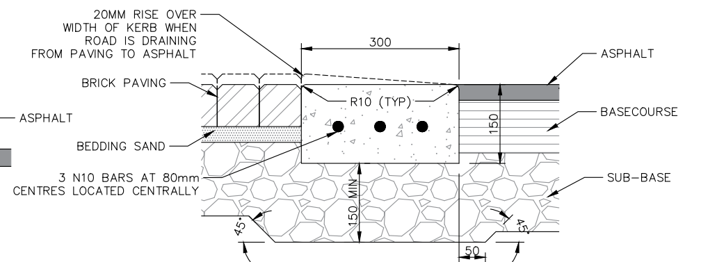
12 Flush Kerb Type FK1
