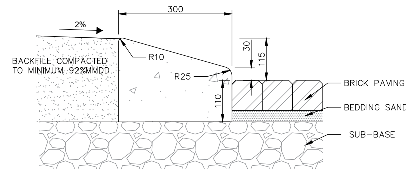
8 Mountable Kerb with Brick Paving Type MK4
